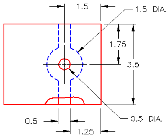
Multiview Drawing
